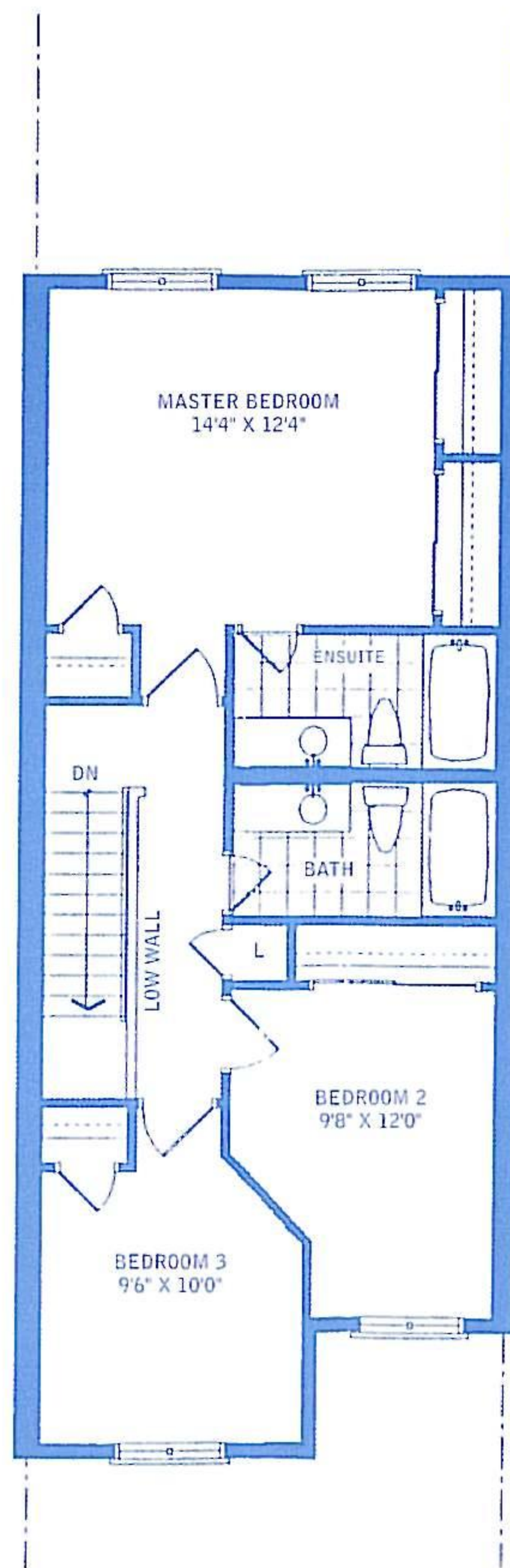
SECOND FLOOR
