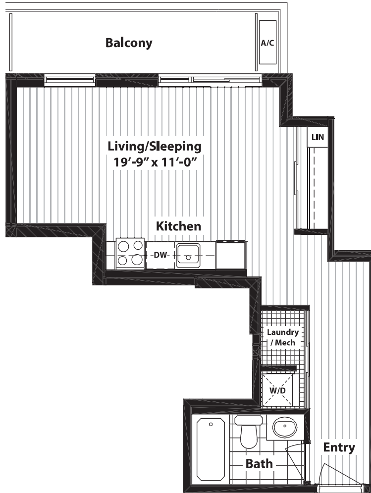
FLOORS 2-4
