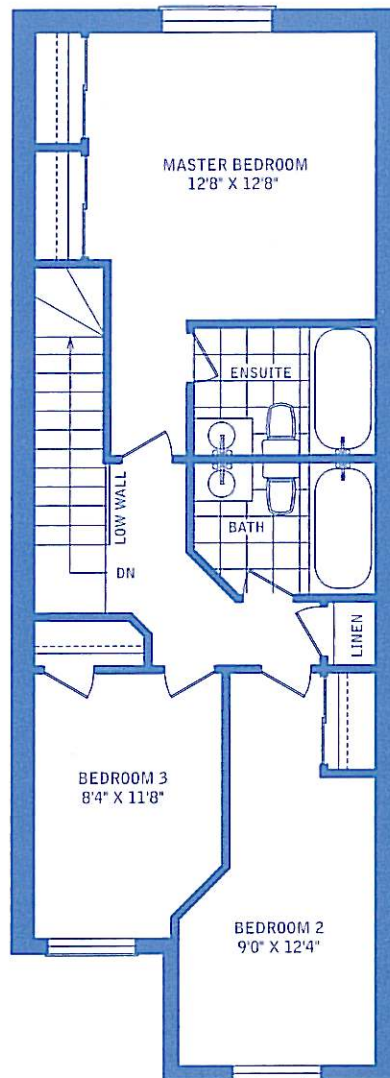
SECOND FLOOR
