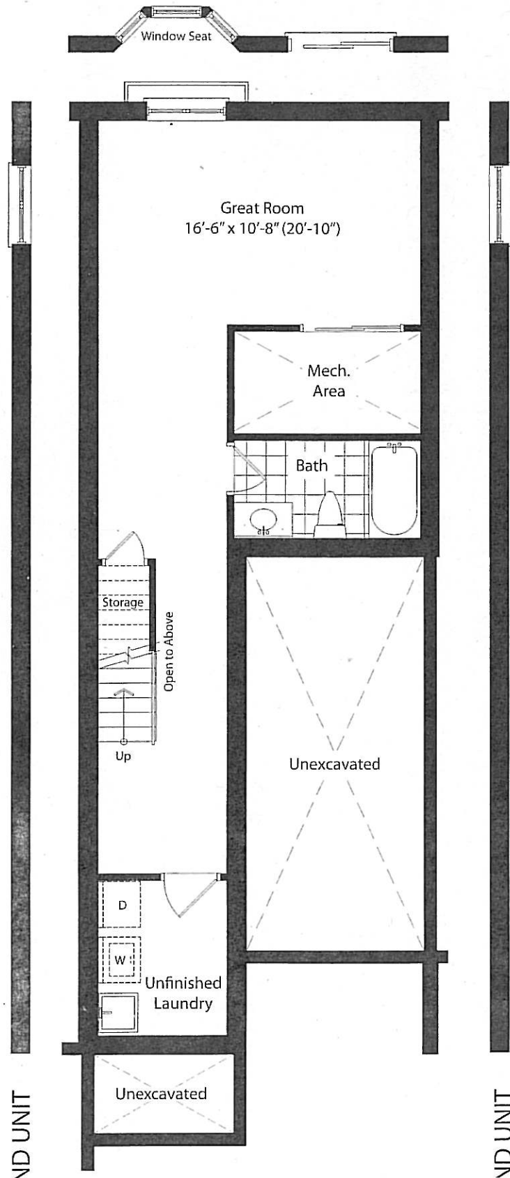
WALK-OUT OPTION
