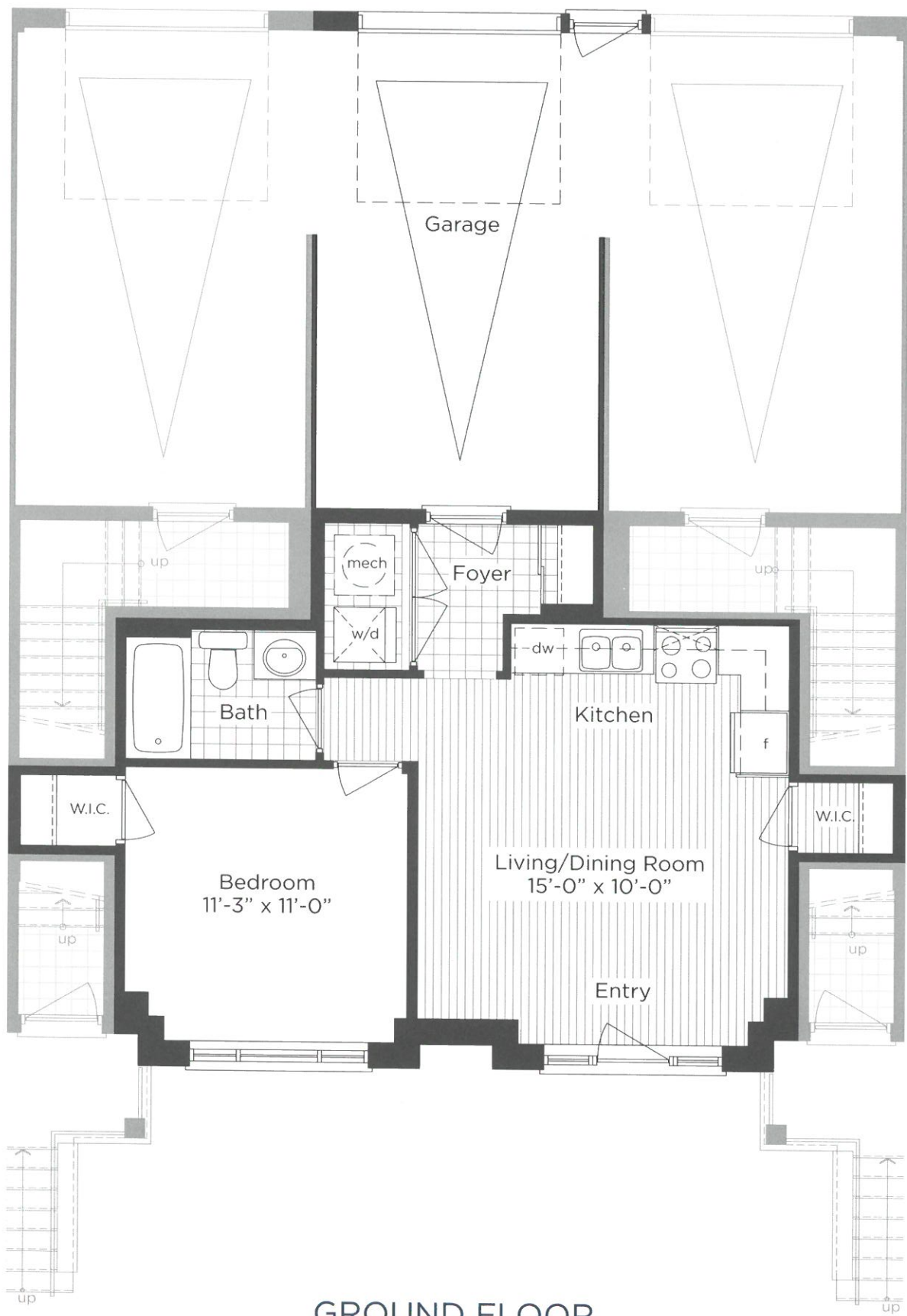
GROUND FLOOR
